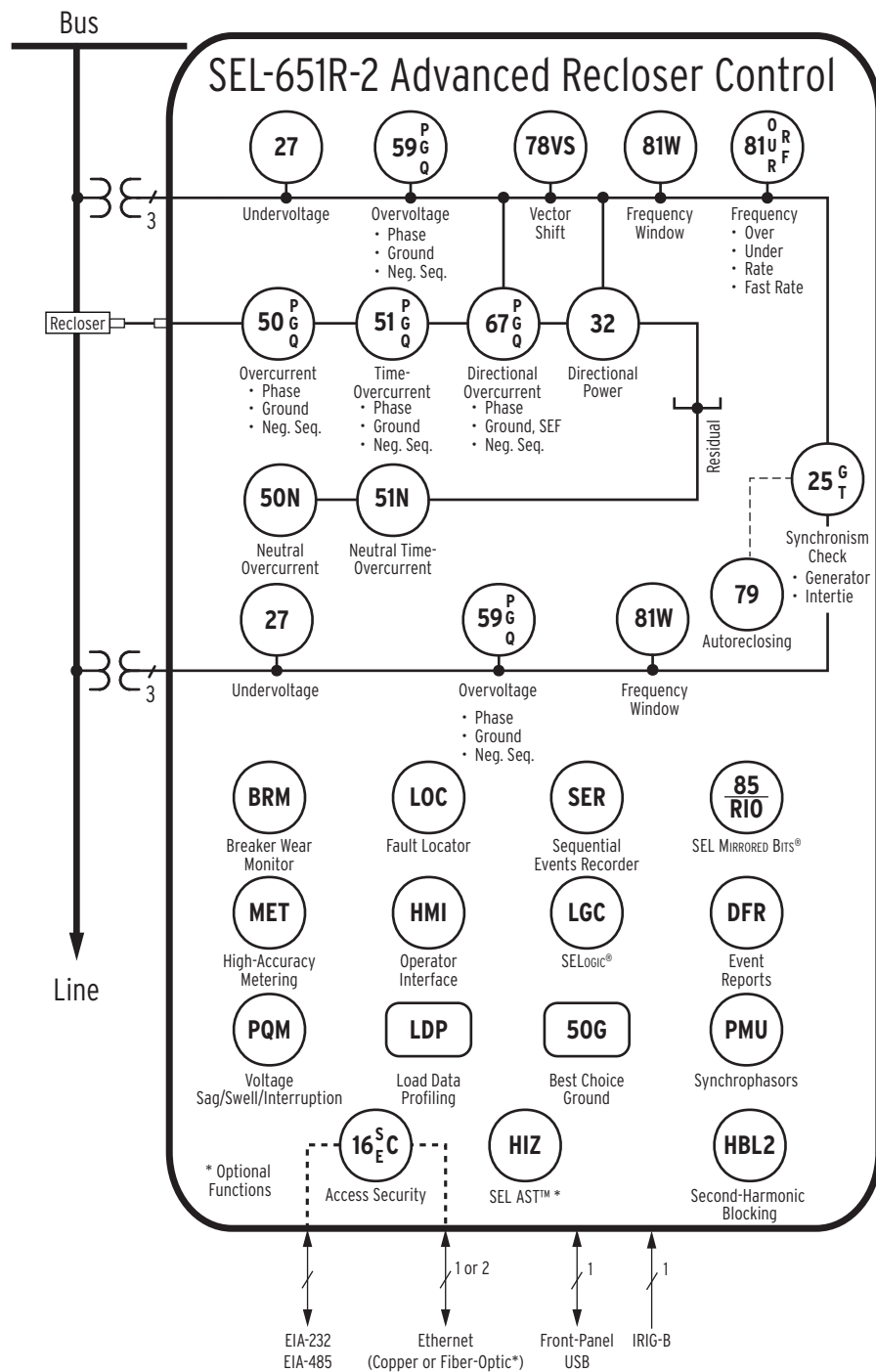
Figure 1 Functional Diagram
