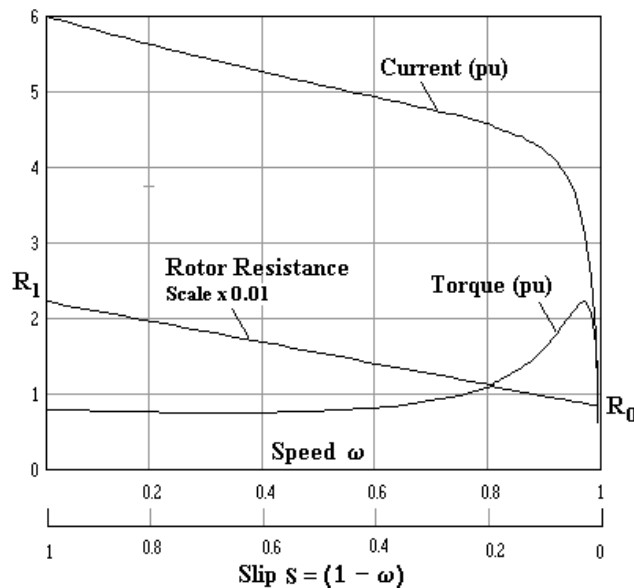
Figure 1: Current, Torque, and Rotor Resistance of an Induction Motor Versus Speed
