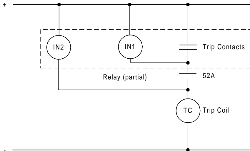
Figure 16: DC Connections for Trip Circuit Monitoring.
