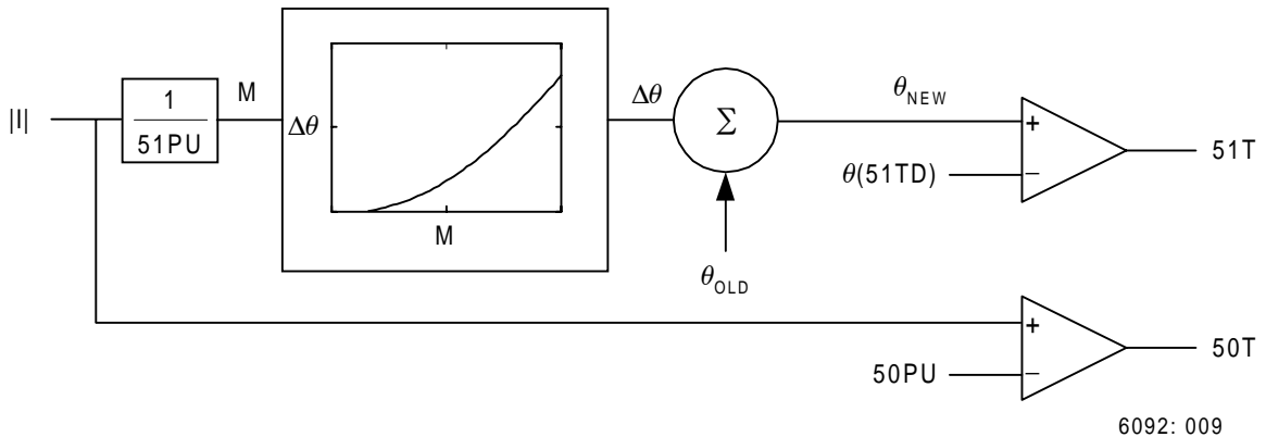
Figure 10: Block Diagram Showing Inverse-Time and Instantaneous Overcurrent Elements.
