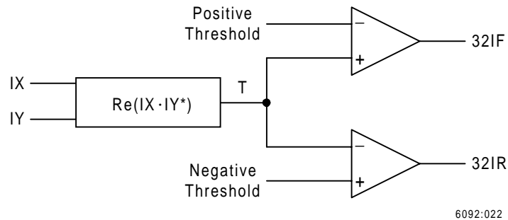
Figure 7: The 32I Directional Element Compares the Angle Between the Residual Current, IX, and the Neutral Current, IY, to Discriminate Between Internal and External Fault Conditions.
