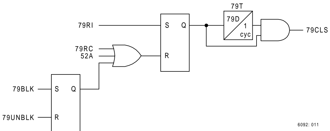
Figure 12: Reclosing Scheme Providing One-Shot Reclosing Following a Feeder Trip.
