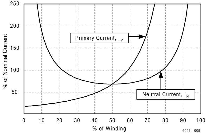
Figure 5: Current Magnitudes Depend Upon the Fault Winding Locations.
