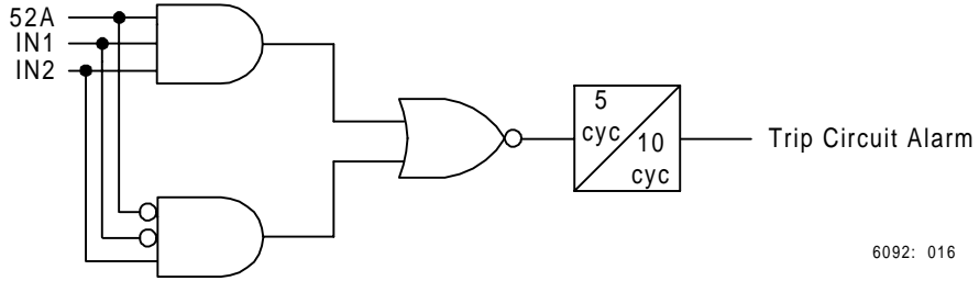
Figure 17: Logic for Detecting Problems in the Breaker Trip Coil.
