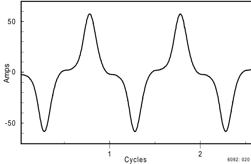
Figure 21: Exciting Current During 150% Transformer Overvoltage Condition.
