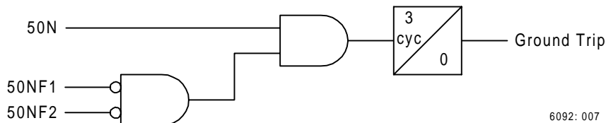
Figure 9: Definite-Time Neutral Overcurrent Element Provides Fast Ground Fault Detection.
