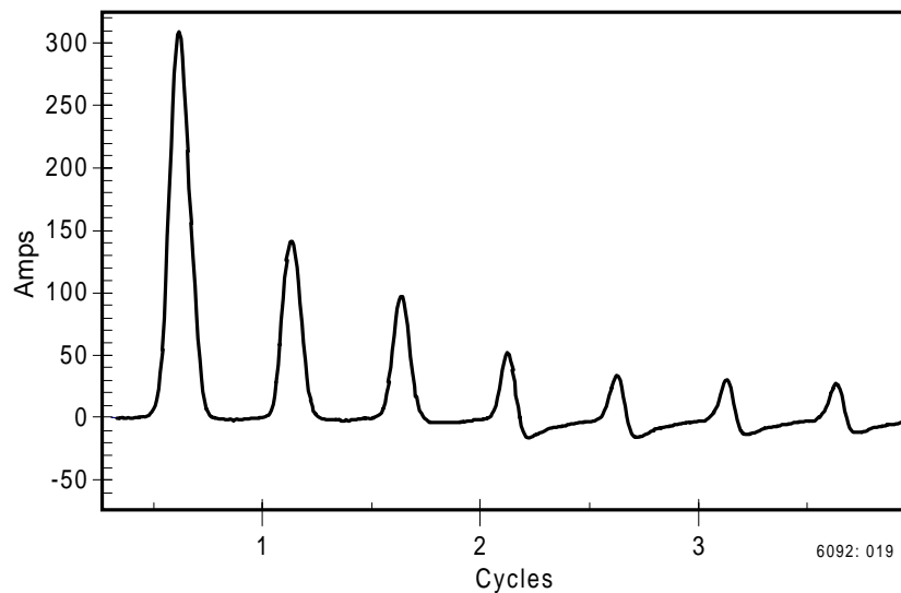
Figure 20: Inrush Current Upon Energization of a Laboratory Transformer.
