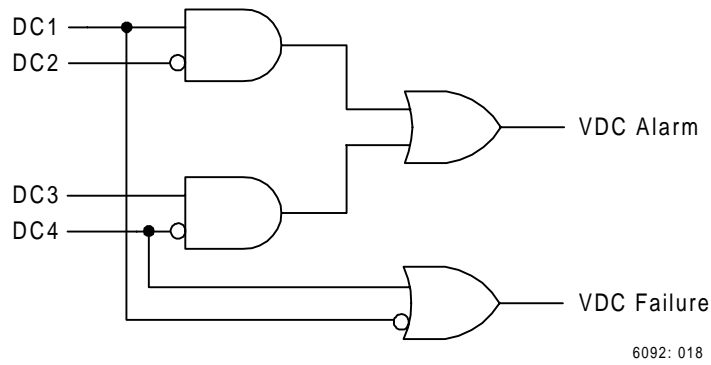
Figure 19: Logic Detects Alarming or Failure Conditions in the Station DC Battery.
