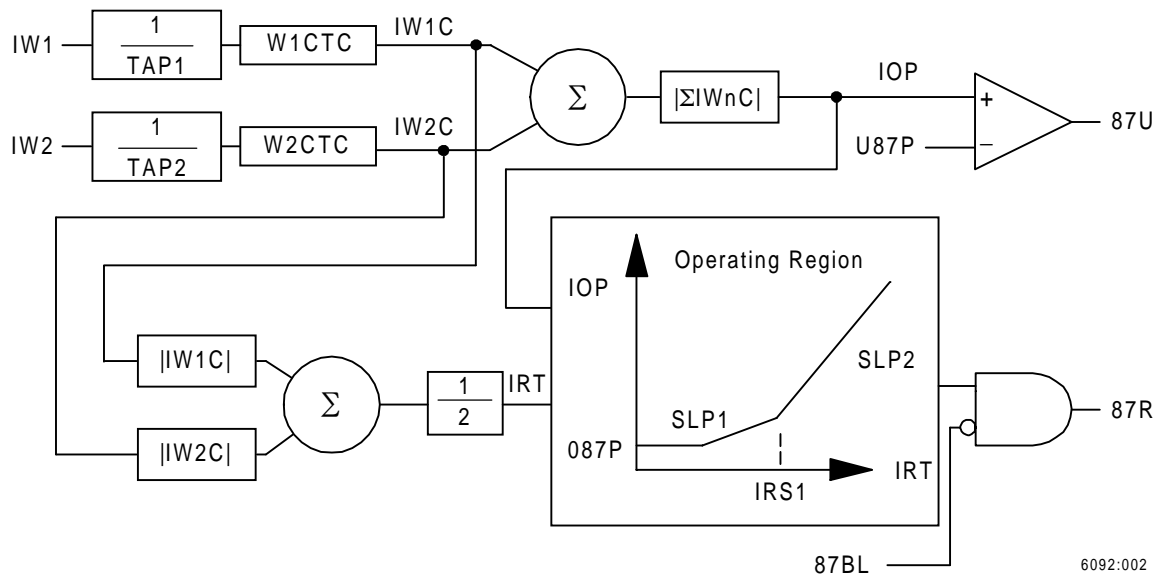
Figure 2: Restrained, 87R, and Unrestrained, 87U, Current Differential Elements for a Two-Winding Transformer.
