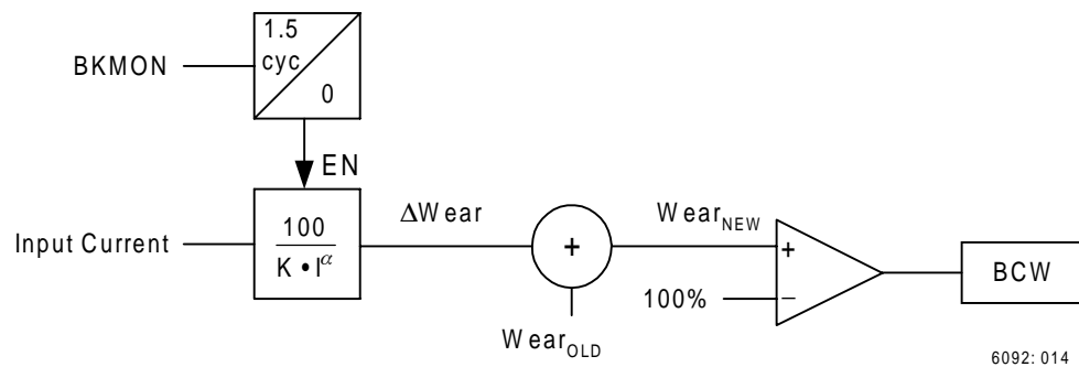
Figure 15: Breaker Wear Monitor Calculates the New Wear Percentage One-and-a-Half Cycles After the BKMON Asserts to Keep Track of the Breaker Contact Wear.
