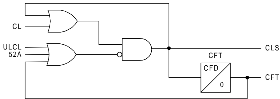
Figure 13: Close Logic With a Close Failure Alarm to Indicate Problems in the Breaker Closing Circuit or Mechanism.
