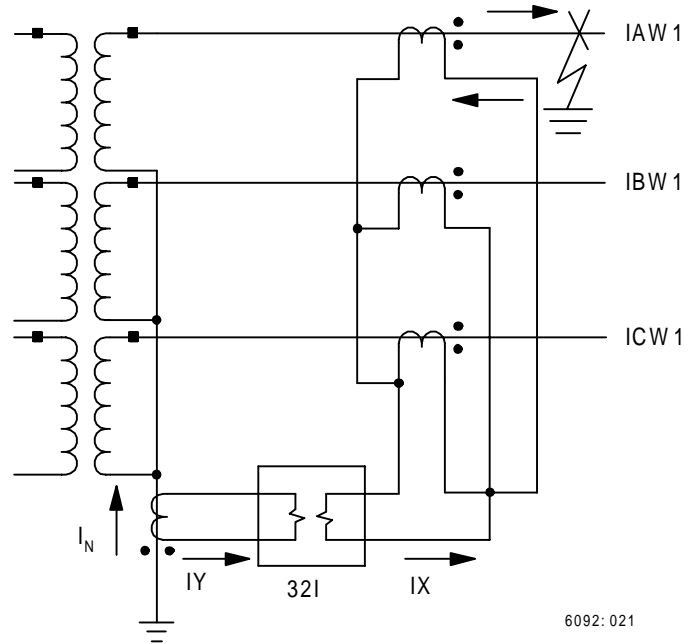
Figure 6: Current Directional Element (32I) for Ground Fault Protection in the Grounded Winding.
