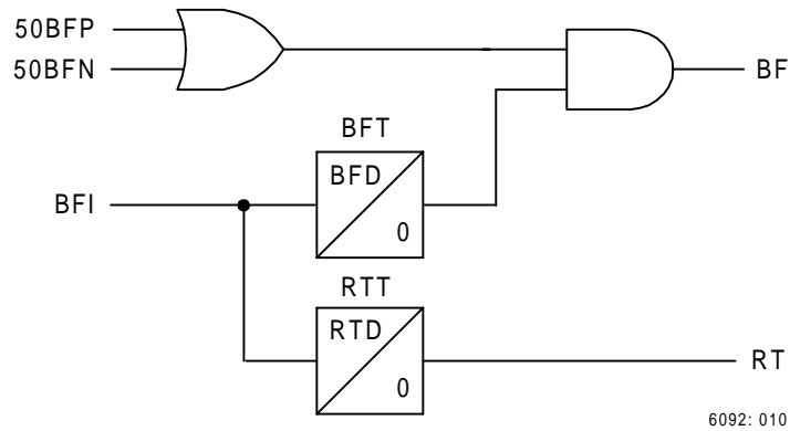
Figure 11: Breaker Failure Logic for Interrupting Fault Currents and Breaker Retrip.
