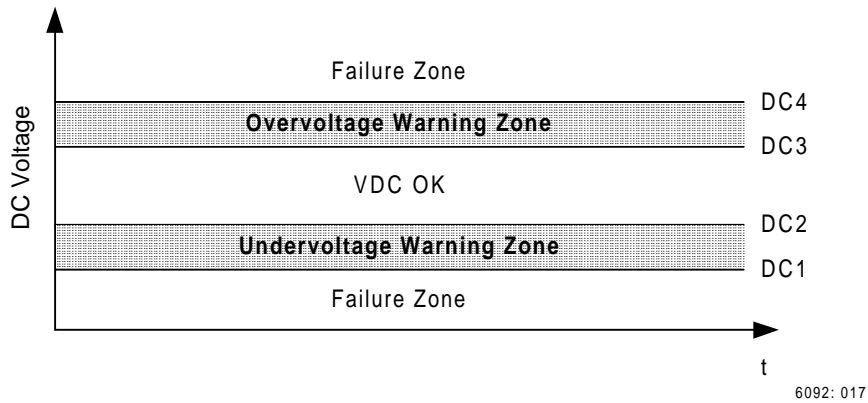
Figure 18: Through Use of Warning and Failure Zones, the Battery Monitor Can Detect Problems in the Station Battery or Charger System.
