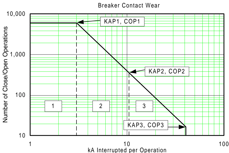
Figure 14: Breaker Contact Wear Curve Shows Low-, Medium- and High-Current Interruption Regions.
