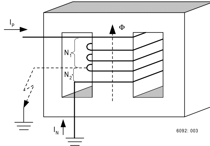
Figure 3: The Neutral Current, I_N , is Proportional to the Phase Current, I_P , for Ground Faults in a Grounded Transformer Winding.
