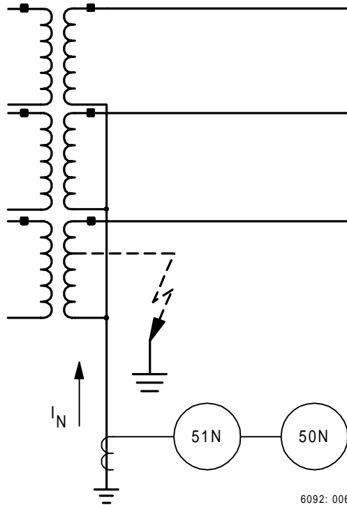
Figure 8: Neutral Transformer Overcurrent Protection Detects Faults Close to the Transformer Neutral.
