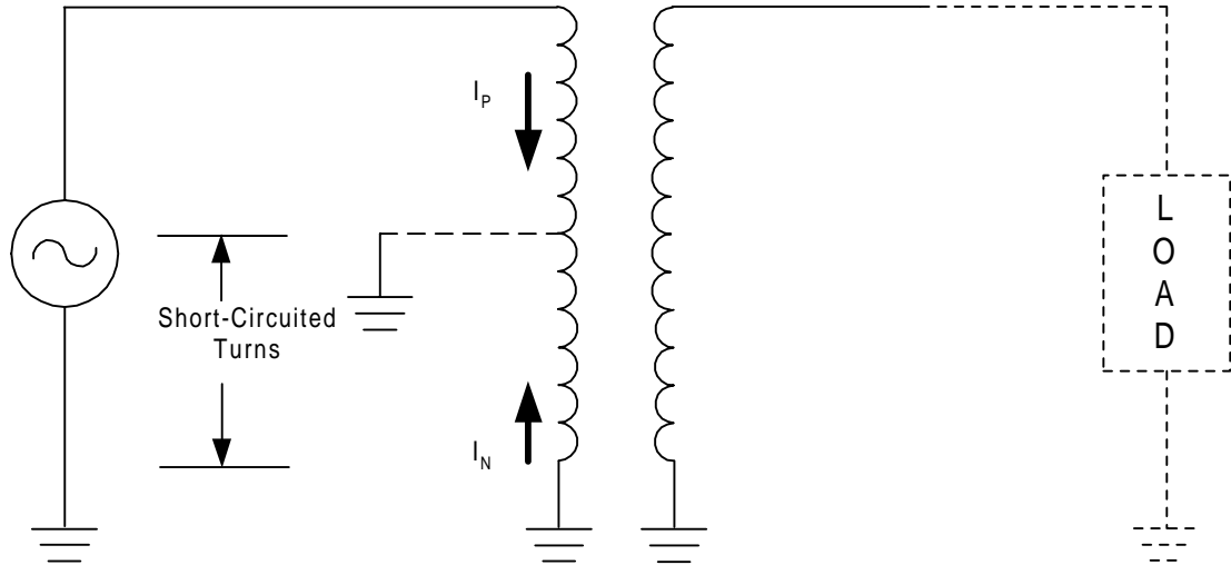
Figure 4: Transformer Ground Faults Produce High Neutral Currents.
